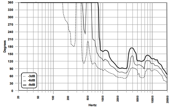
Vertical Beamwidth
