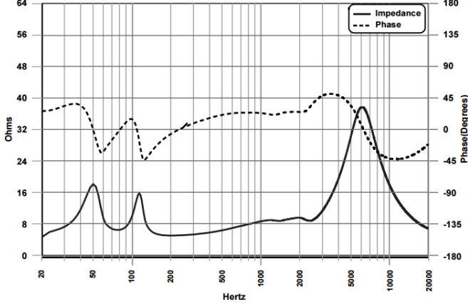
Phase/Impedance
